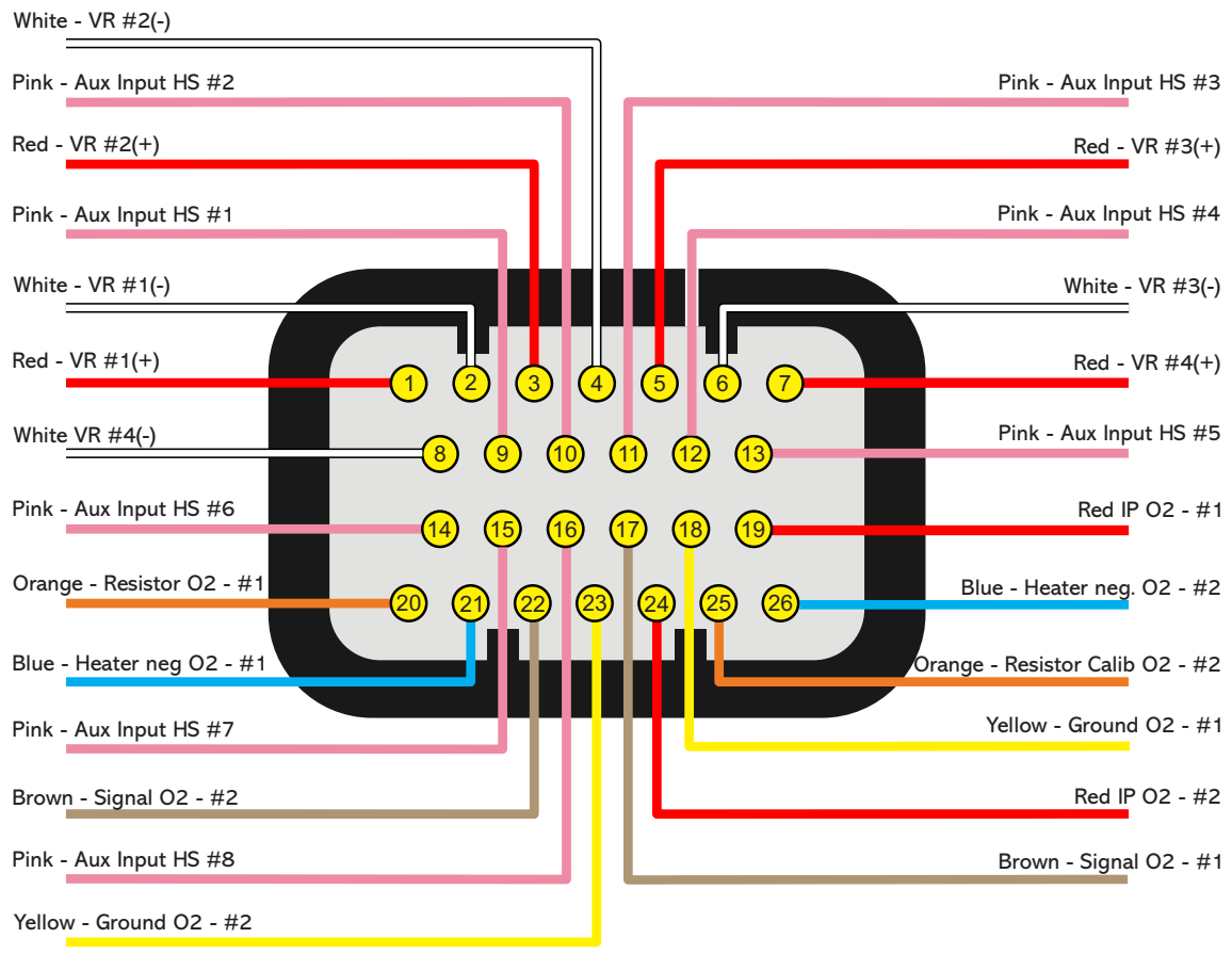
Harness connector rear view
