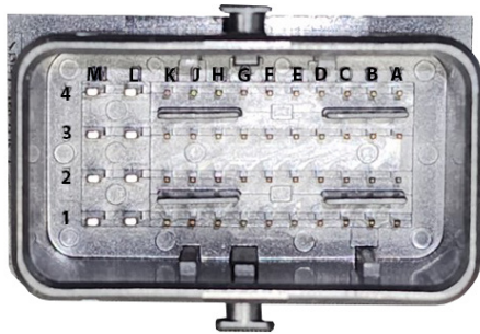
Conector B
