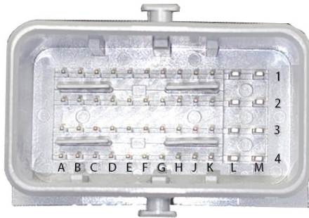
Conector A
